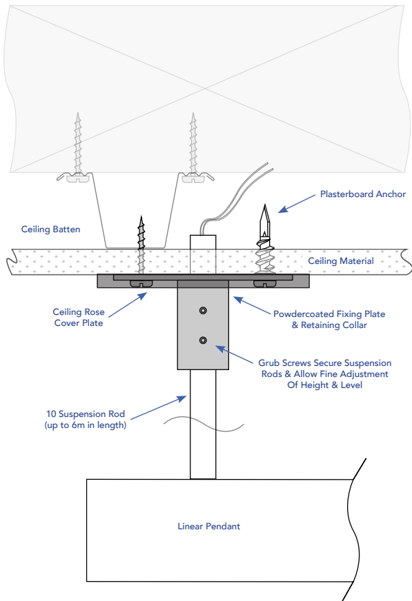
Flat Ceiling Installation Method
