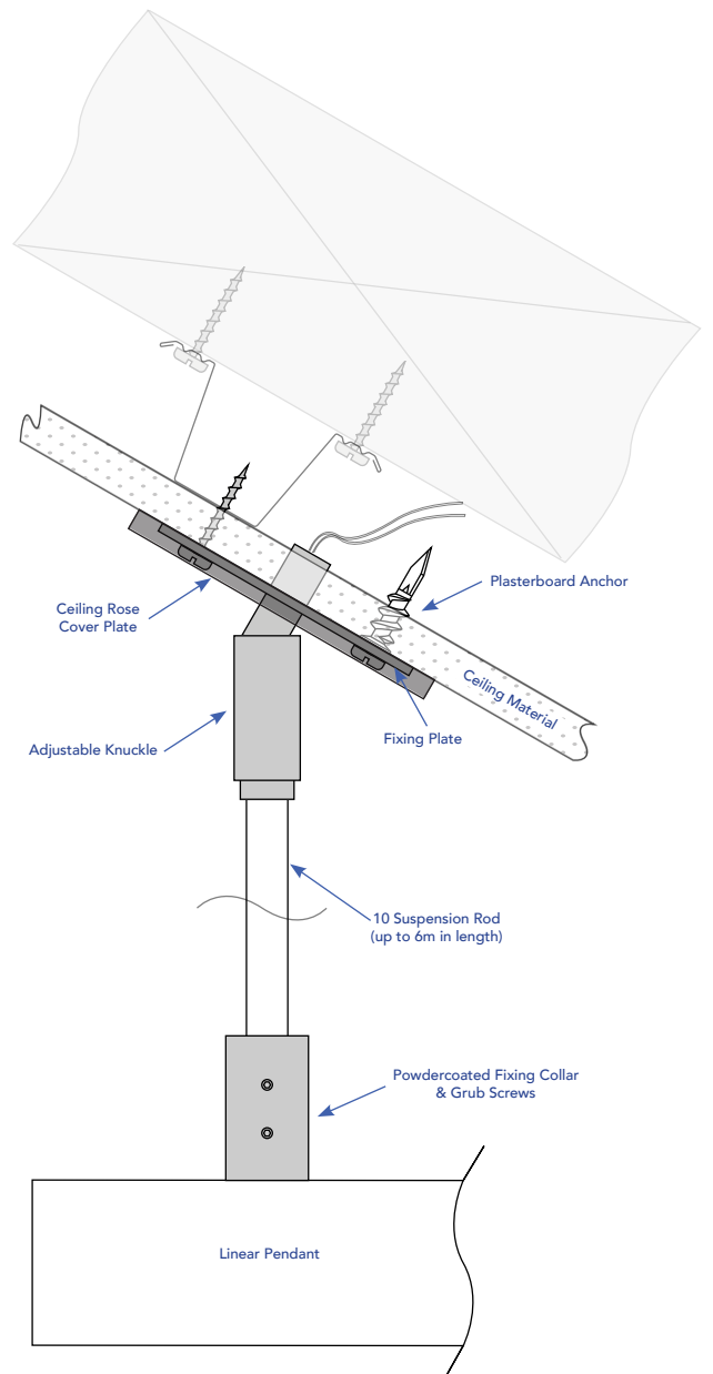
Raked Ceiling Installation Method
