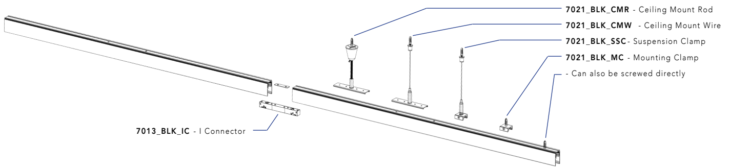
7021_BLK_CMR - Ceiling Mount Rod
