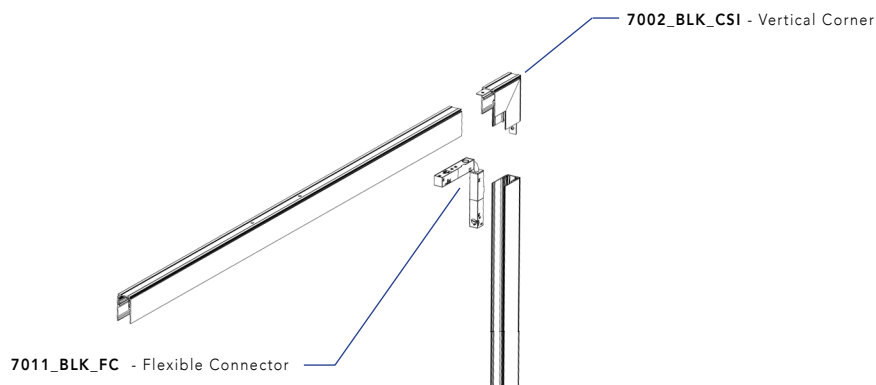
7002_BLK_CSI - Vertical Corner
