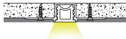
Typical Installation
